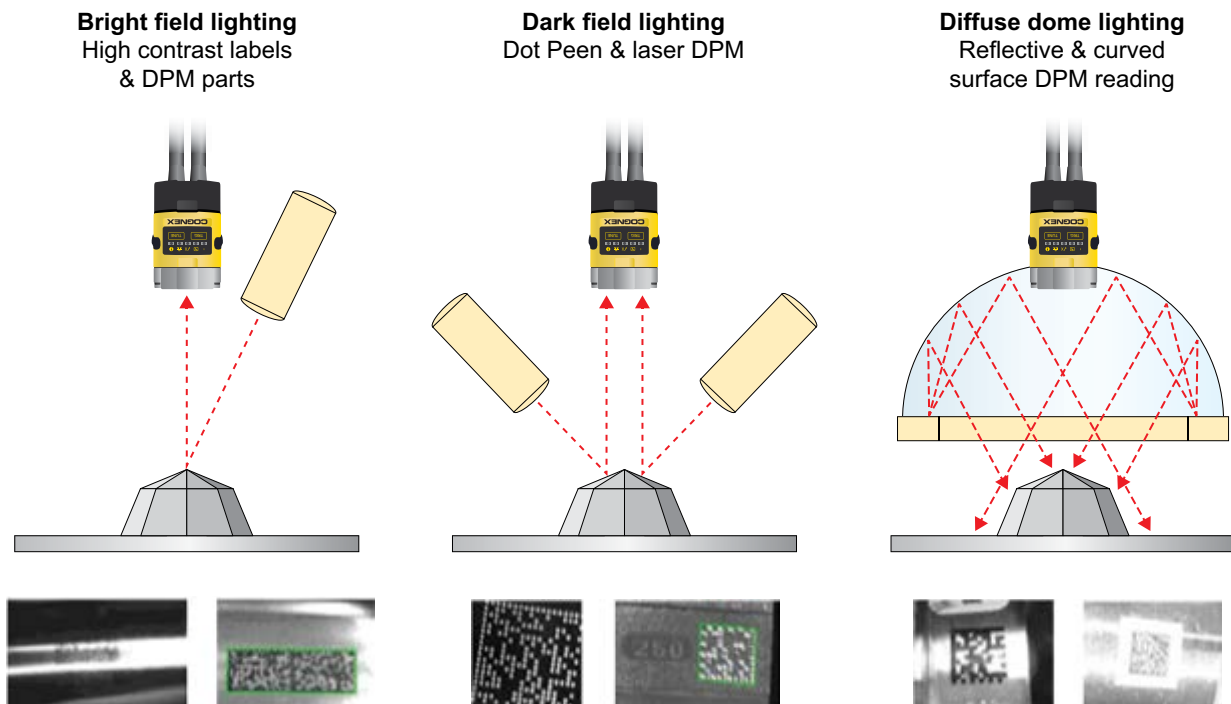
Figure 17: Lighting technology
